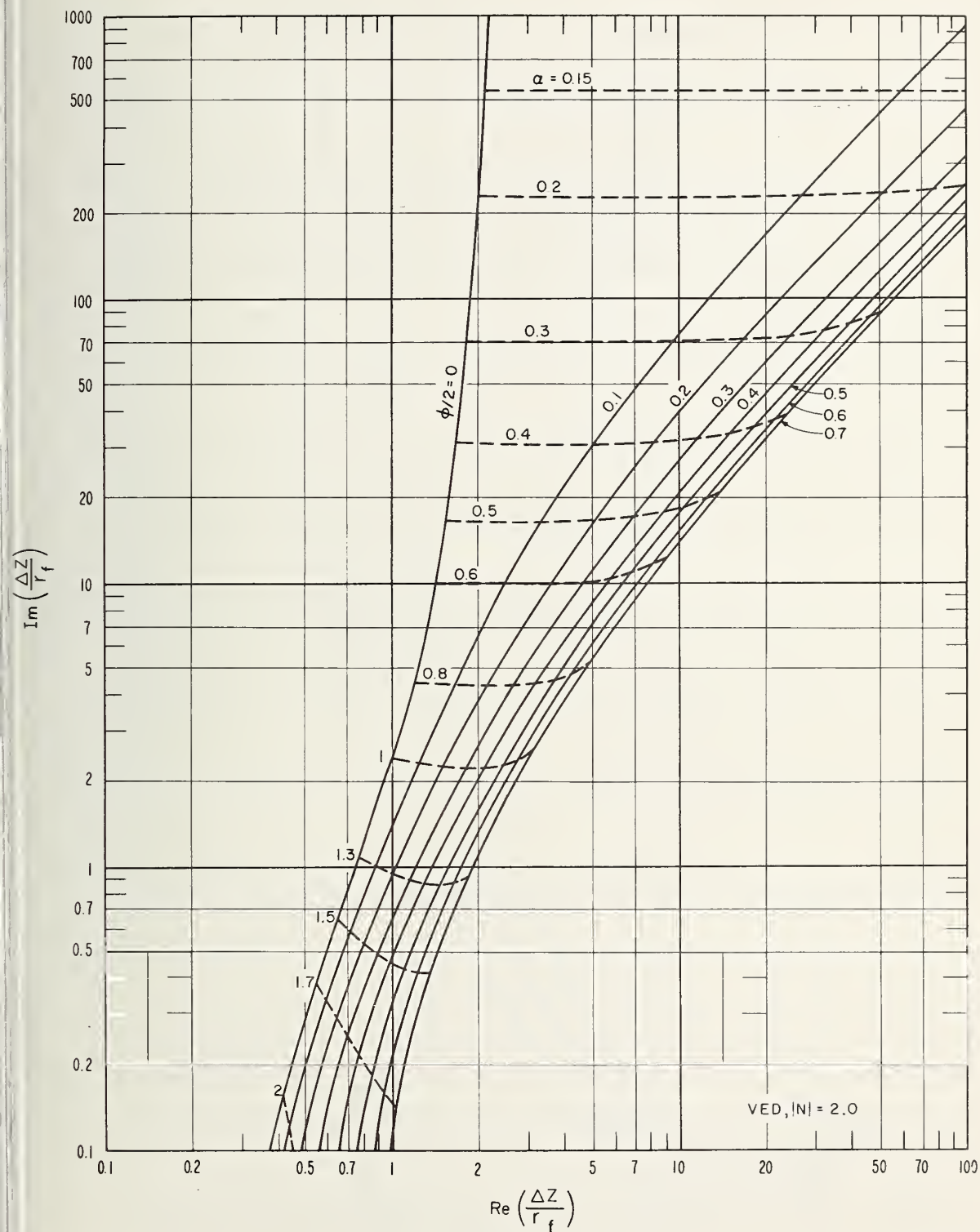
Figure A-32. Normalized input impedance change for VED, |N| = 2.0 .
